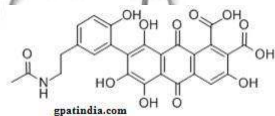
laccaic acid
